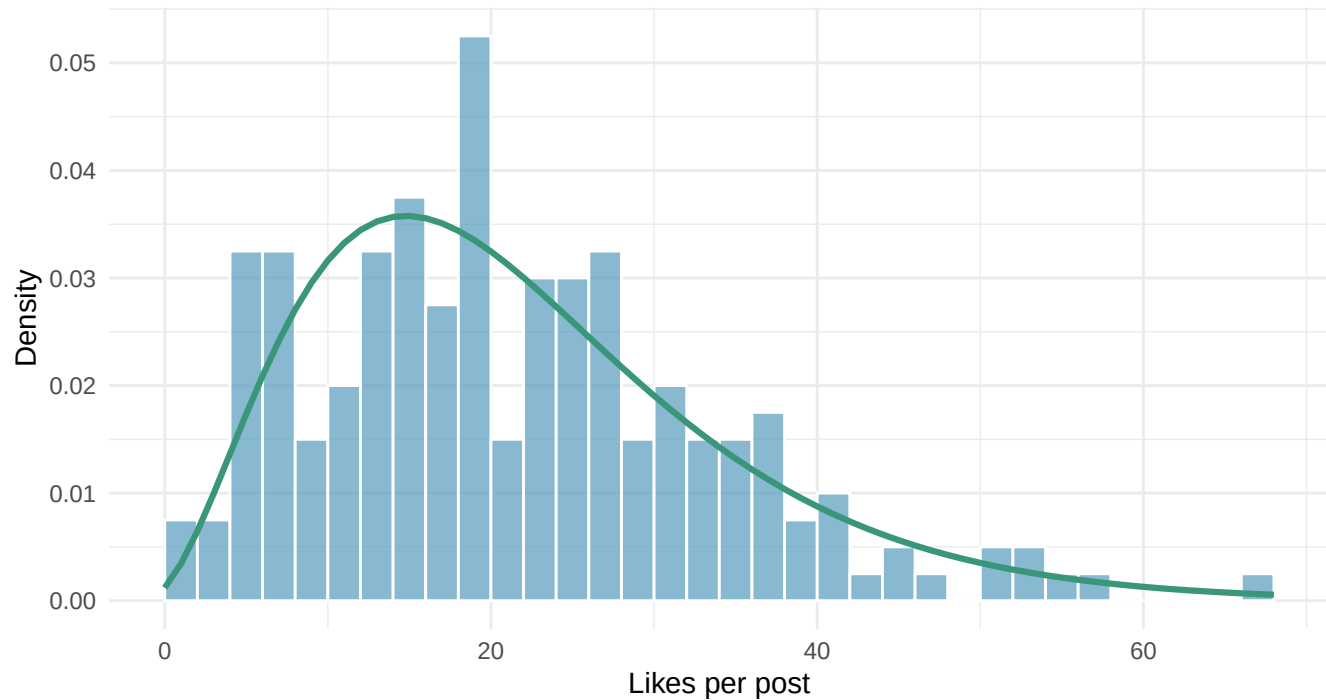
Negative Binomial MLE fit ( \hat{\mu} = 21.9 , \hat{\text{size}} = 3.32 )
