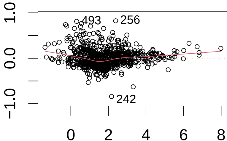
Residuals vs Fitted
