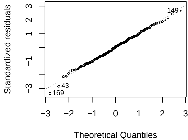
\log(y) : \log(y) \sim x
