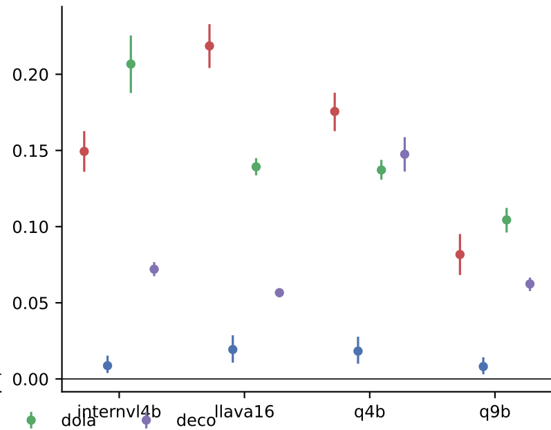
high-accuracy stratum
