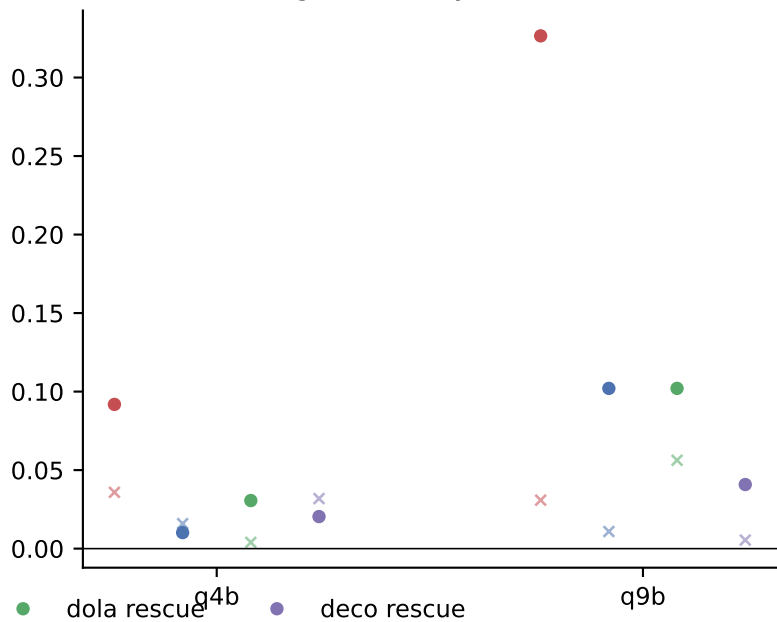
high-accuracy stratum
