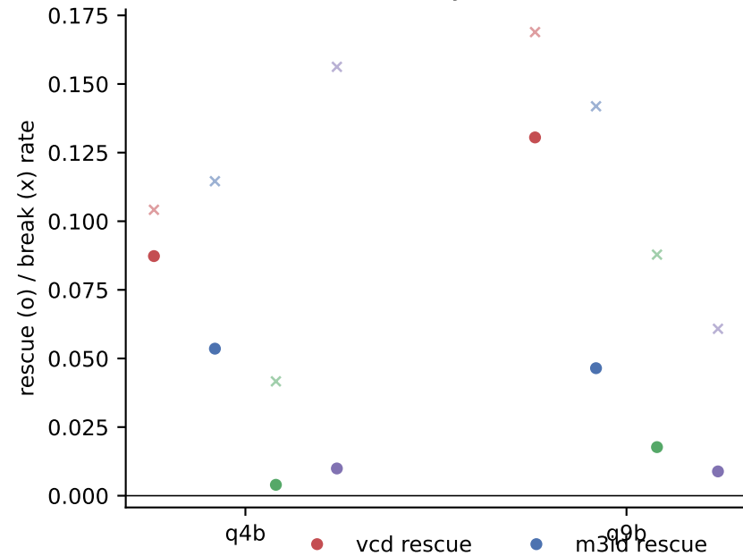
low-accuracy stratum
