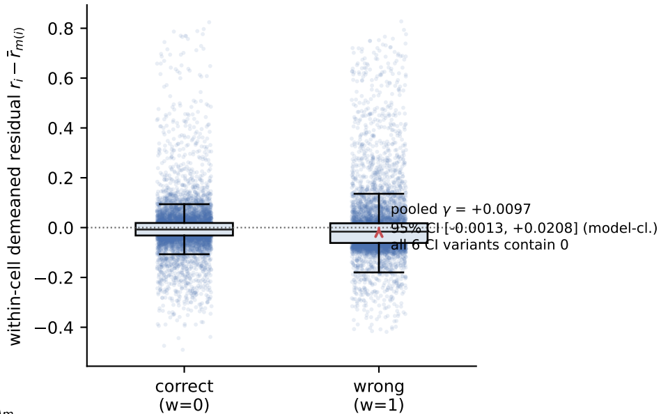
(b) residual distribution by answer correctness (cell fixed effects removed)
