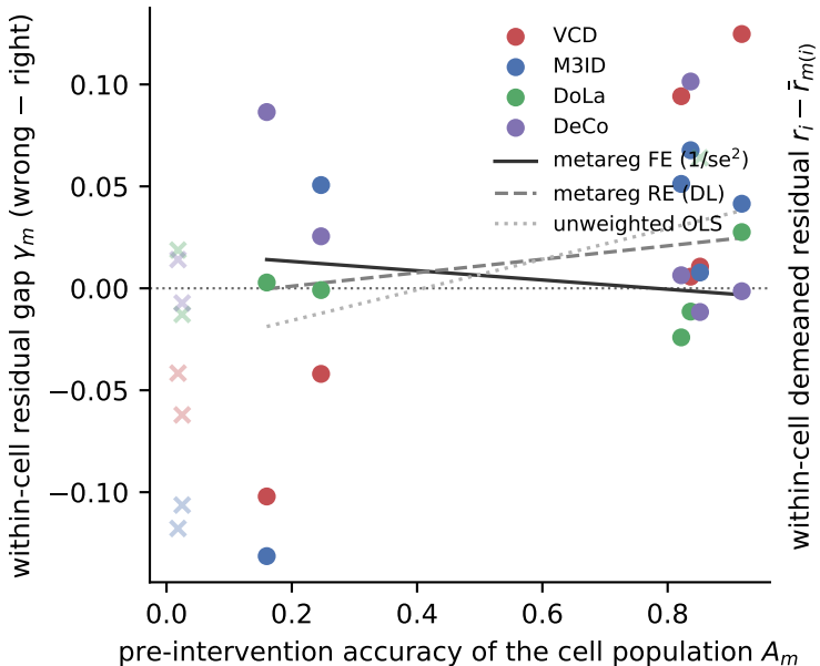
(a) per-cell residual gap vs population accuracy (x = stage-7 insufficient cells)
