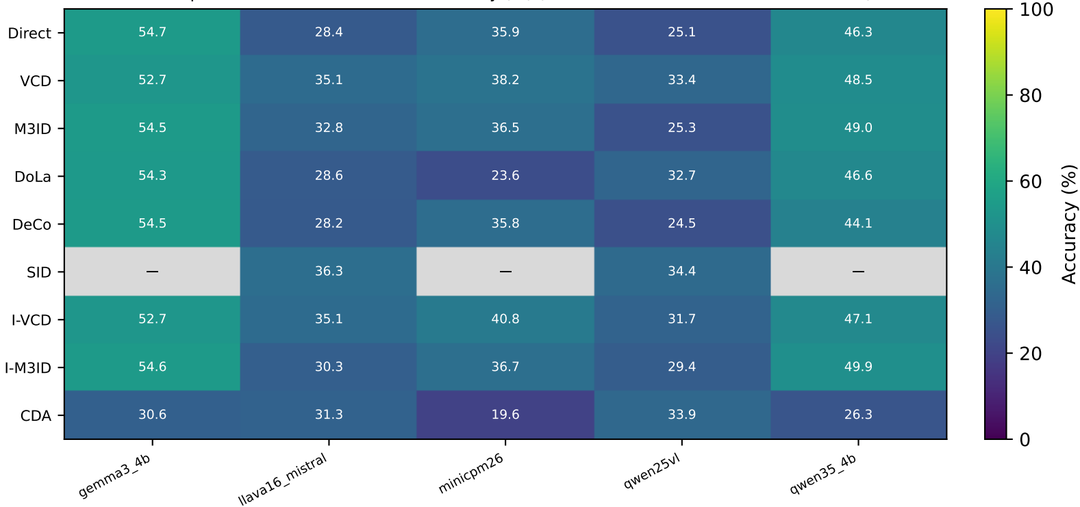
Descriptive UNKNOWN/UNKNOWN accuracy (%) (42 exact condition cells; n=2,424 each)
