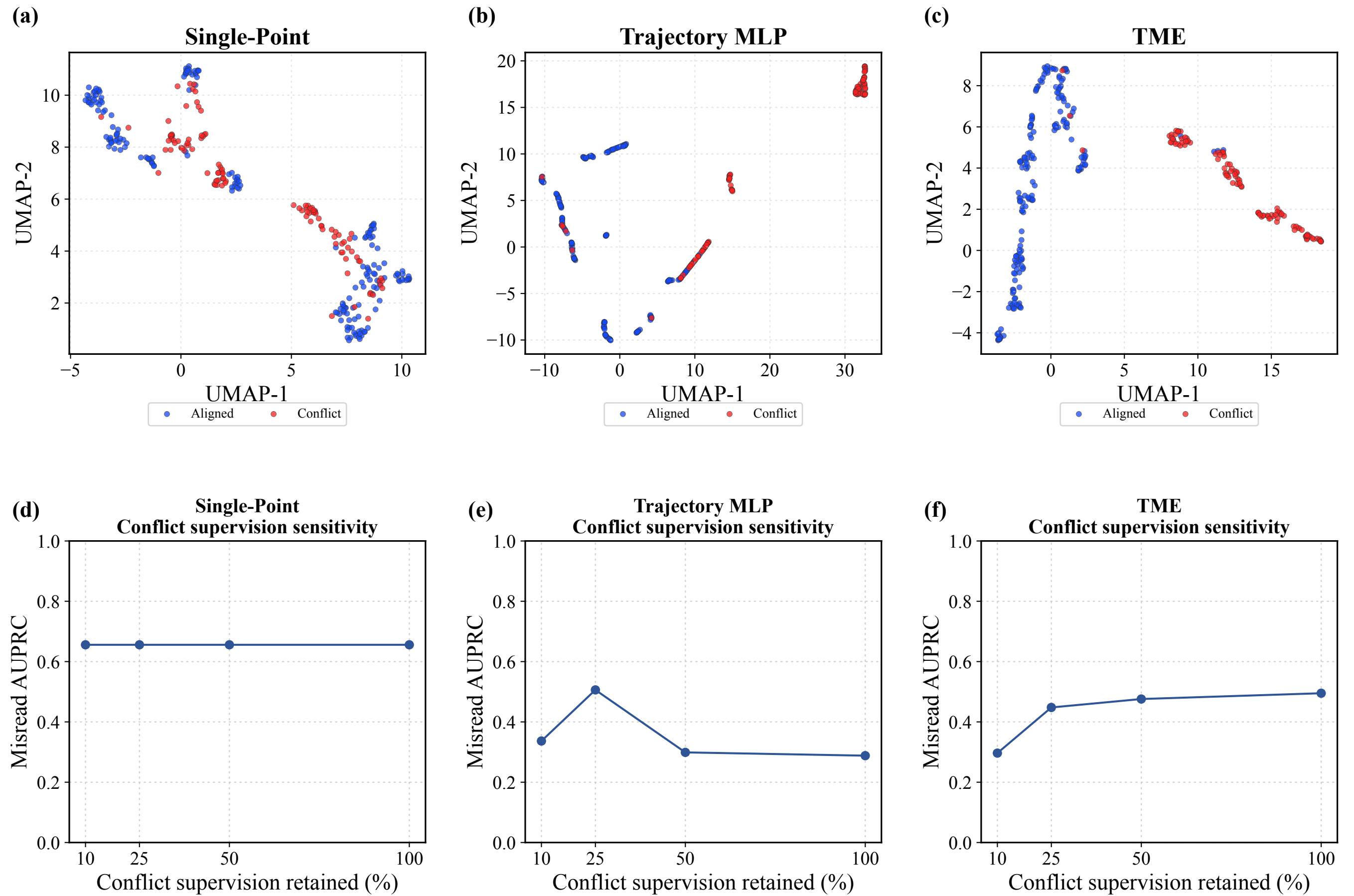
Figure 8. Frozen representation quality and Conflict-supervision sensitivity
