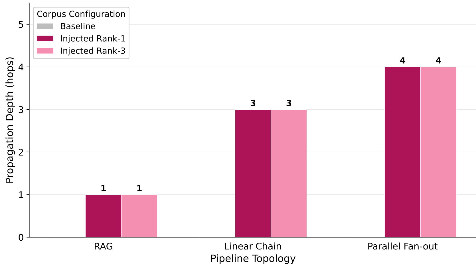
Injection Propagation Depth by Topology and Corpus Configuration
