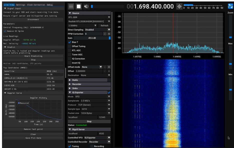
Fig. 5 Identification of SARAL in the L band.
