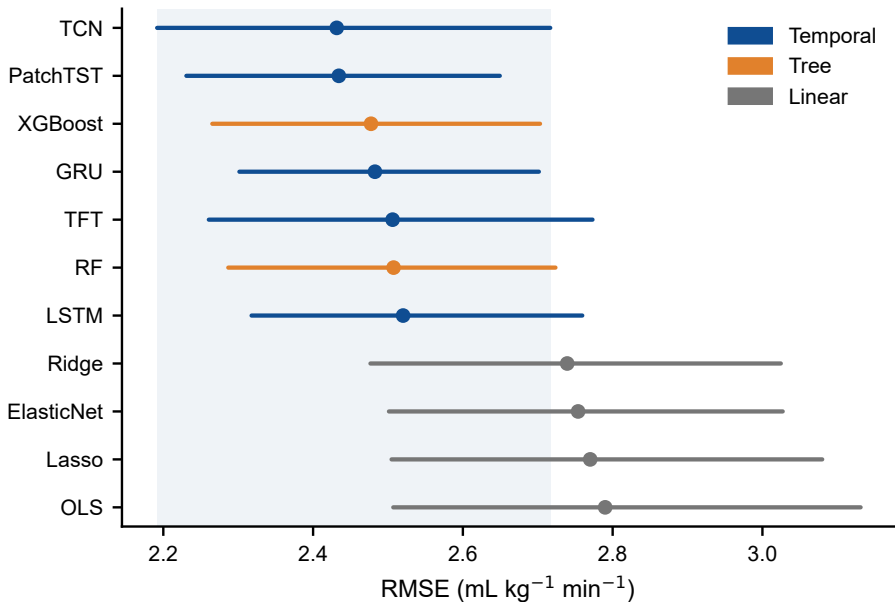
Per-participant mean RMSE with subject-cluster bootstrap 95% CI
