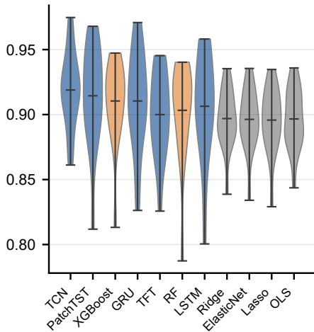
Pearson r
