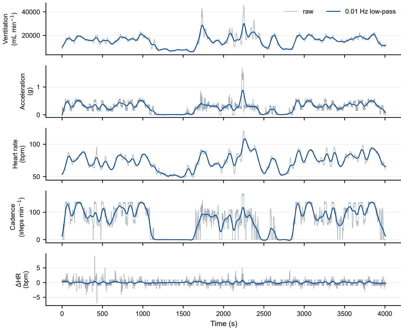
Raw vs. 0.01 Hz low-pass filtered wearable signals (participant 1)
