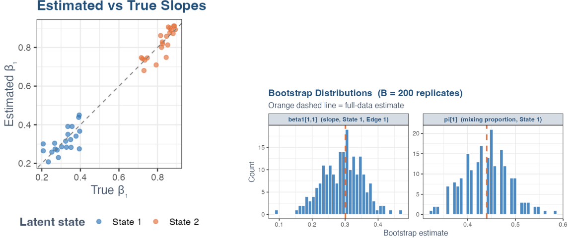
(a) Estimated vs. true slope parameters \hat{\beta}_1 for all q = 21 edges across both states (best-of-20 EM fit; replicates, n = 100 , p = 6 , K = 2 ). Dashed lines = n = 100 , p = 6 , K = 2 . (b) Bootstrap distributions of \hat{\pi}_1 and \hat{\beta}_{1,1}^{(1)} ( B = 200 replicates). Orange dashed line = full-data estimate.
