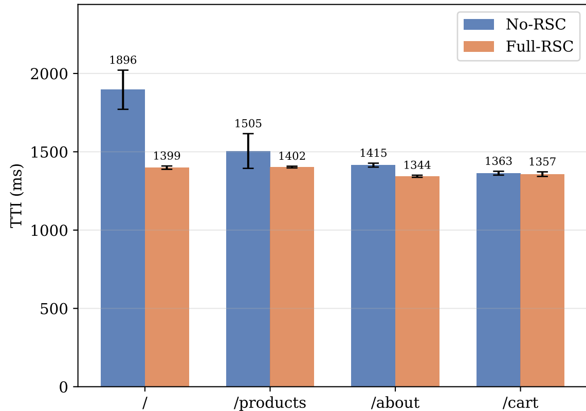
Time to Interactive (TTI)
