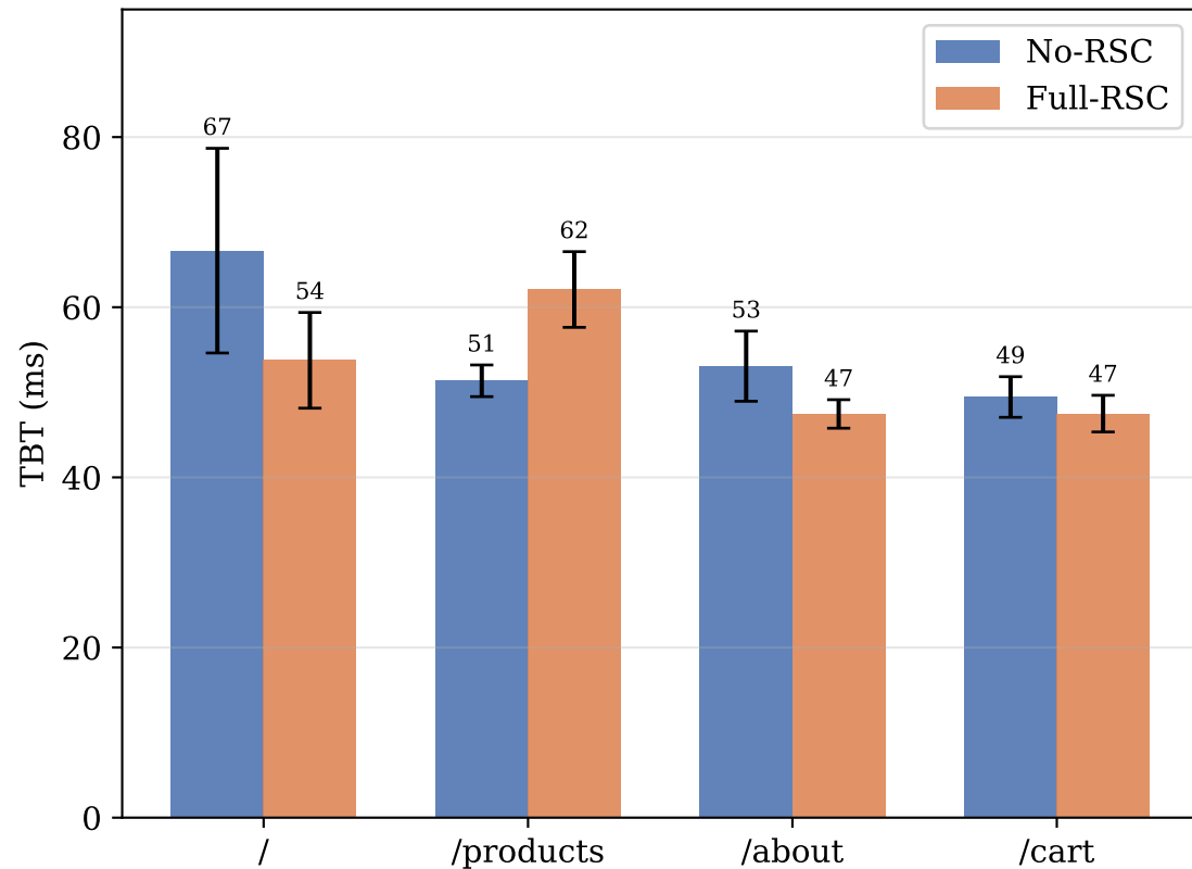
Total Blocking Time (TBT)
