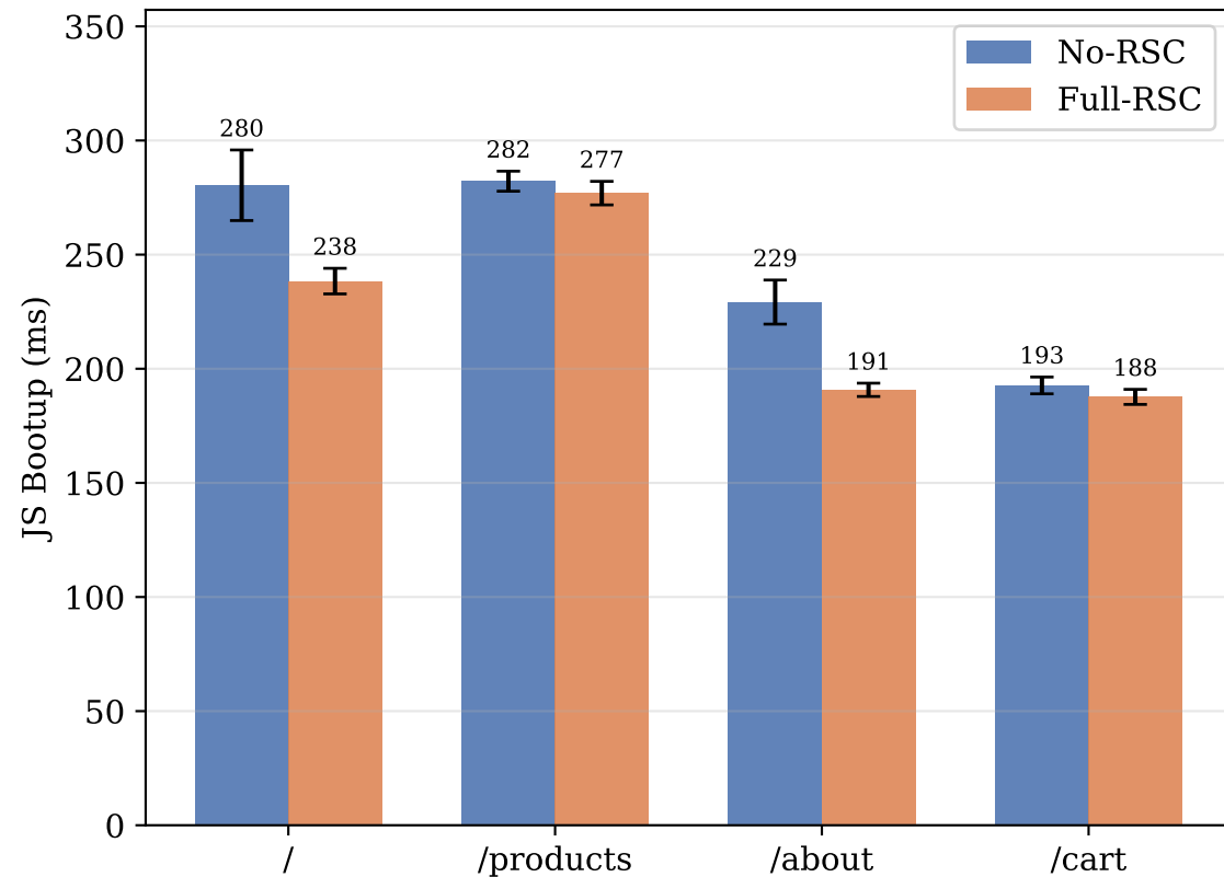
JS Bootup Time
