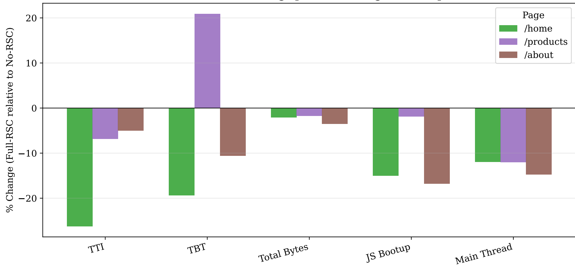
Full-RSC vs. No-RSC: % Change per Metric (negative = improvement)
