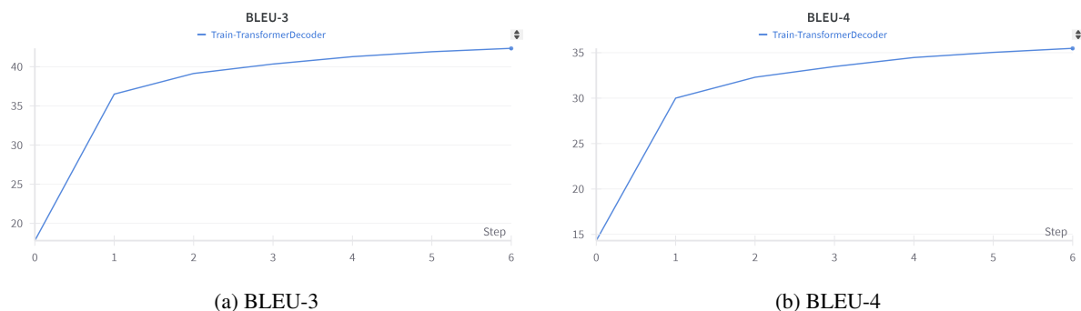
Figure 3: Wandb Training BLEU Score for Model with Post-layer Normalization
