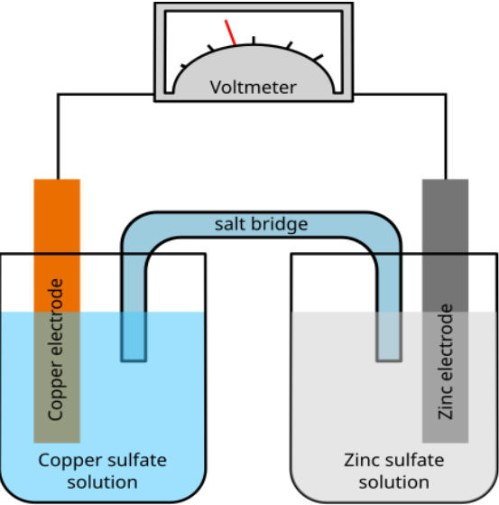
Electrochemical cell
