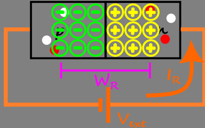
@ Reverse bias
