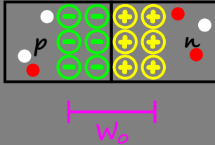
@ Zero bias
