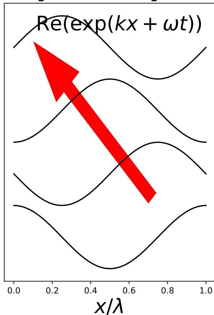
Negative travelling wave
