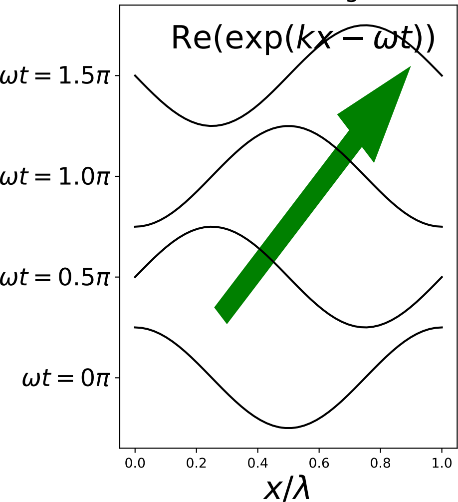
Positive travelling wave
