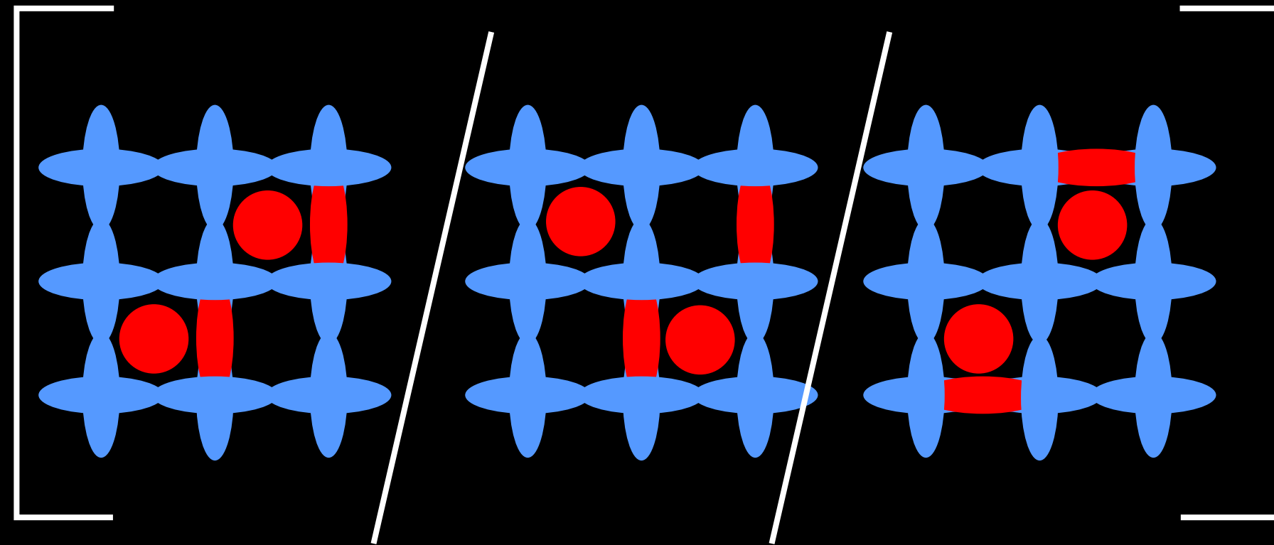
Si covalent solid at finite T
