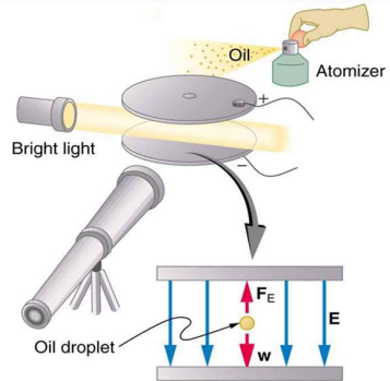
Oil drop experiment
