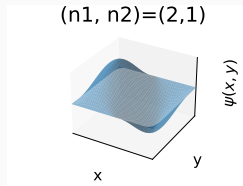
2D wave functions
