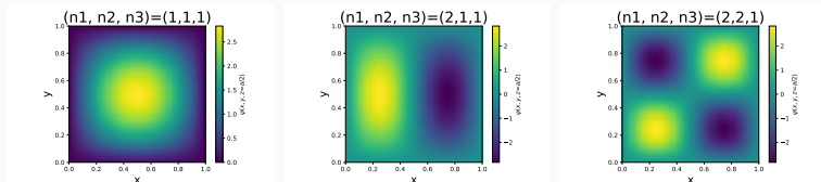
3D wave functions
