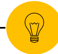
Card Sorting
