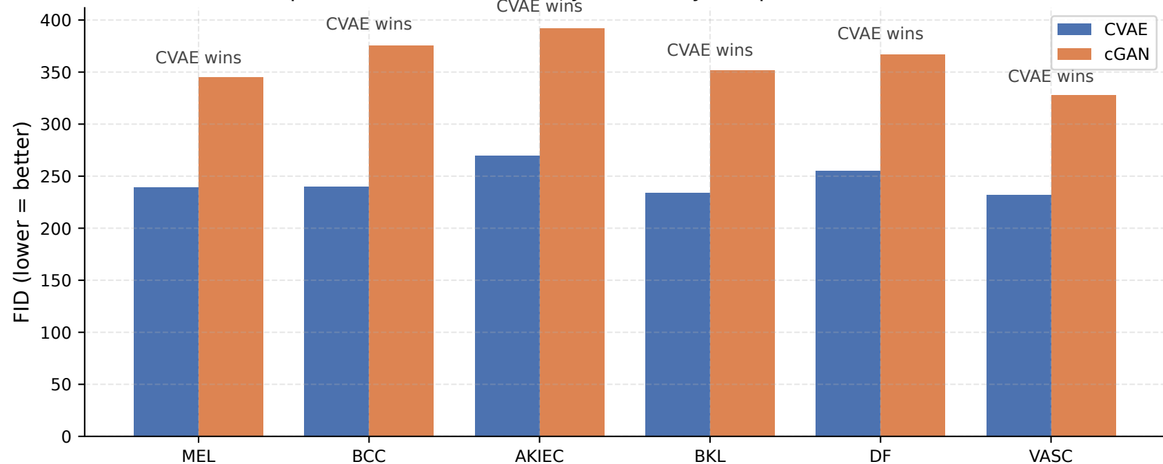
Sample quality per class — CVAE vs cGAN (comparable within a class only; biased by sample size across classes)
