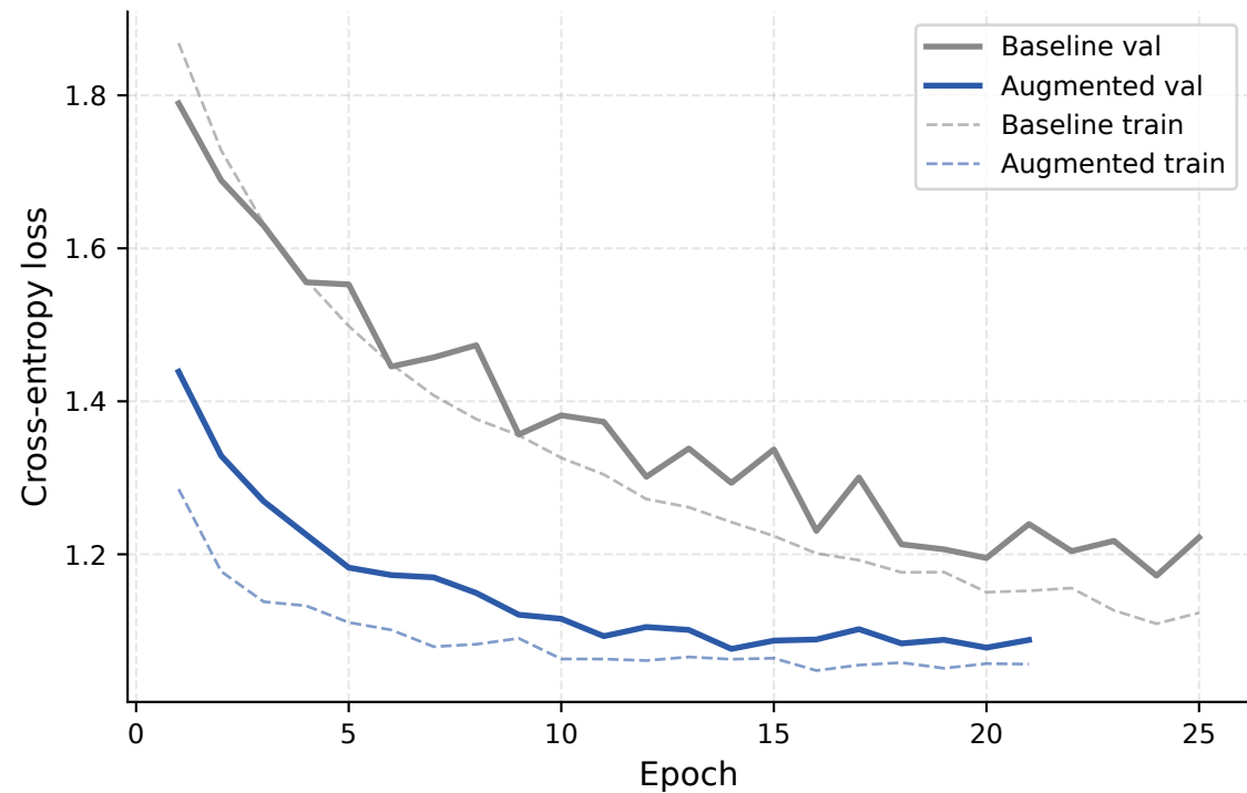
Loss
