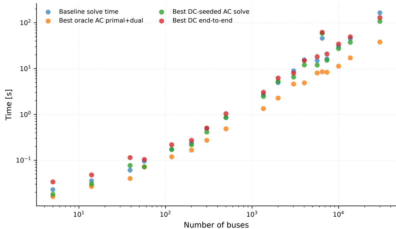
Case size versus runtime
