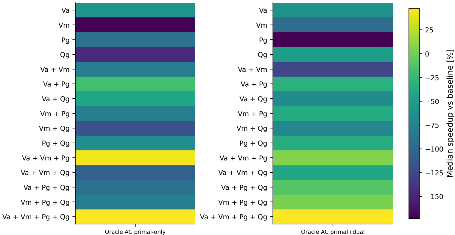
Oracle AC combination heatmap
