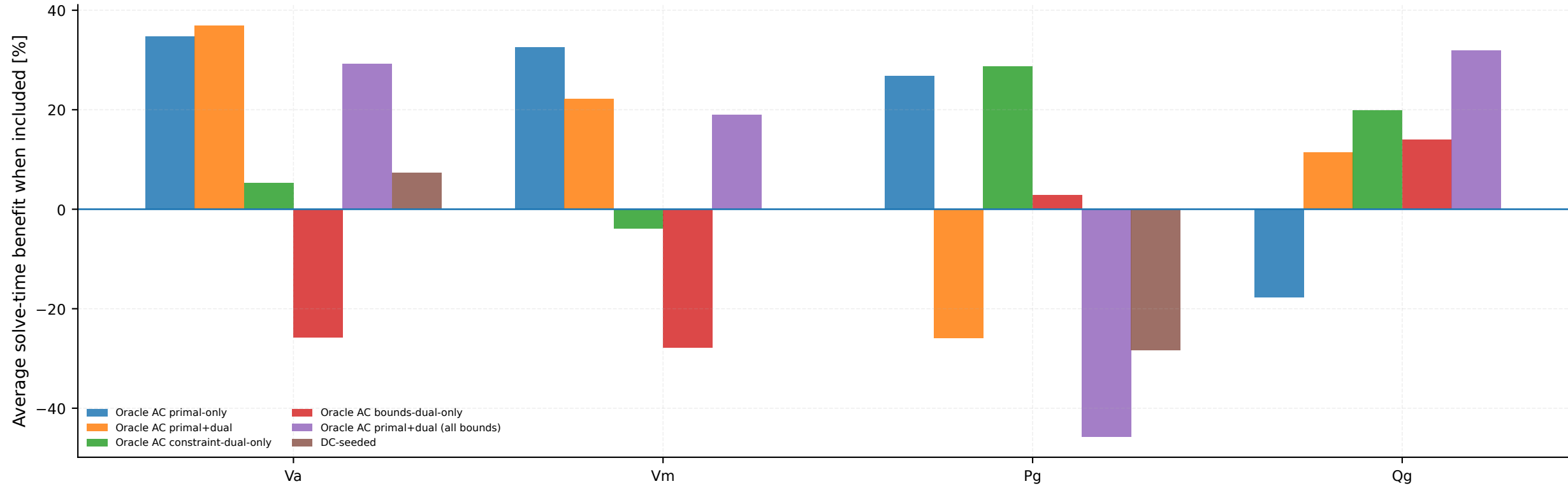
Average benefit of each initialization block
