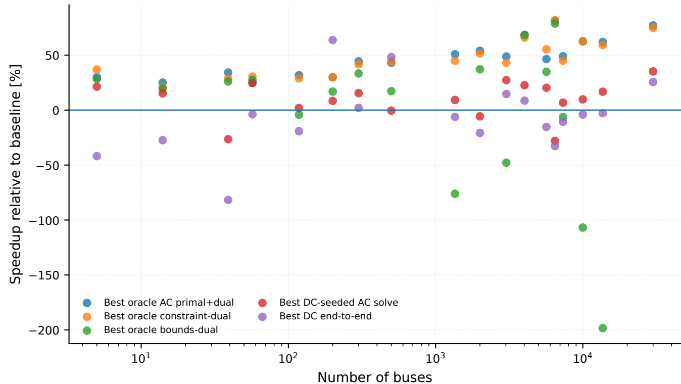
Speedup versus case size
