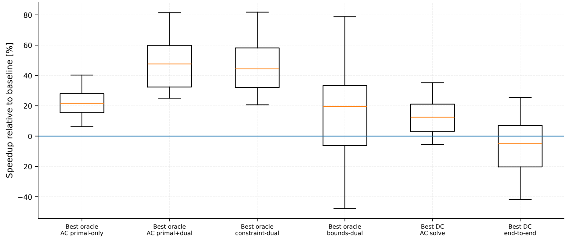
Distribution of per-case speedups
