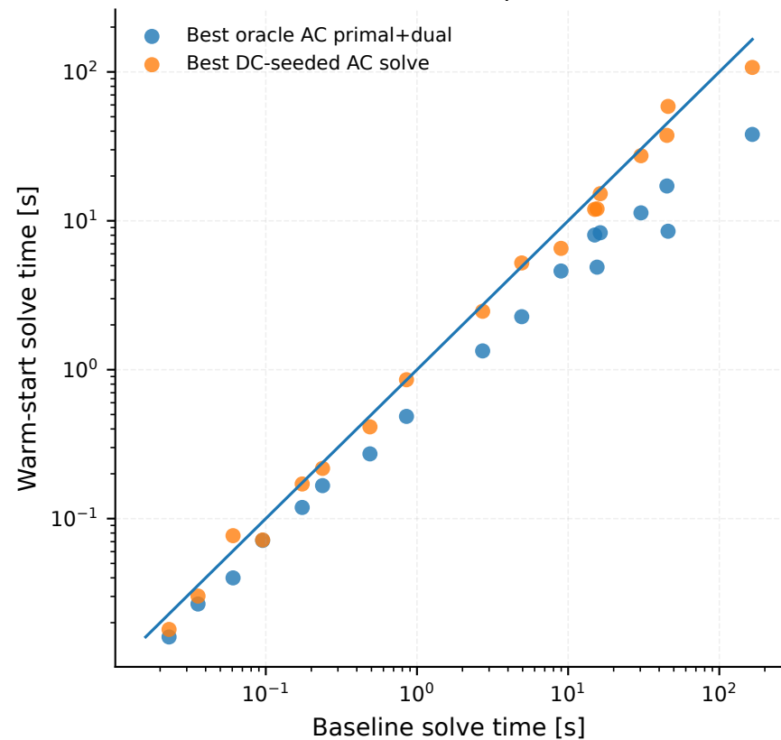
Solve-time comparison
