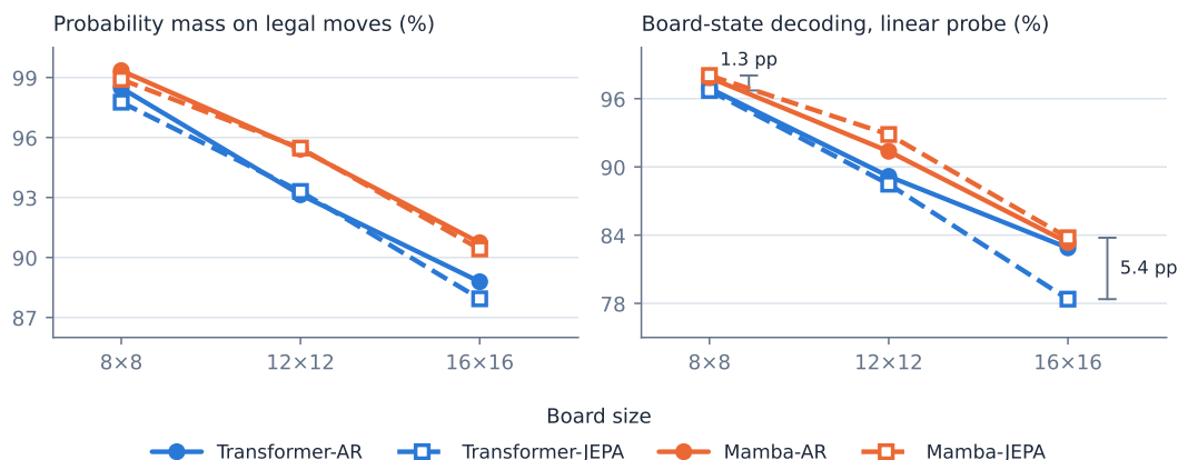
Figure 1: Colour encodes architecture, line style encodes objective. The two Transformer variants separate at 16 \times 16 while the two Mamba variants stay together: the interaction is visible only off the saturated scale.
