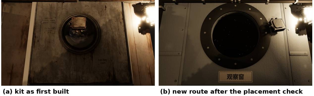
Figure 6: A fault caught by the placement check. (a) In the first build of the hub, a conduit box covered the porthole. (b) In the new route, the placement check found the box in front of the opening and moved it 0.5 m along the wall before anything was spent.
