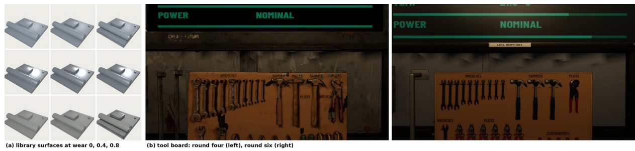
Figure 4: (a) Three surfaces from the shared library (painted panel, bare steel and deck plate) at wear settings 0, 0.4 and 0.8. (b) The hub's tool board when each generated piece kept the colours of its own picture (left), and after every surface came from the library and each tool became its own model (right). Both shots use the same camera and the same build of the game.
