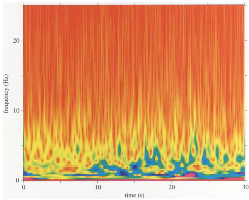
Figure 9. The Morlet wavelet spectrum for the wind data with the same number of frequency cells. Wind energy appears in smoothed contours with a rich energy distribution in the high harmonics.
