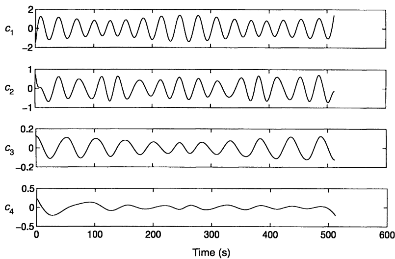
Figure 26. The first four IMF components after stringent application of EMD. There are up to 3000 siftings for some components. The first components, c_1 , indeed shows 512/30 = 17 waves; while the second components, c_2 , shows 512/34 = 15 waves. The other components are of negligible energy. While the EMD succeeded in extracting the intrinsic time scale of the processes, the components failed to give the exact constant amplitudes and frequencies, a flaw due to the accumulation of errors from the imperfect spline fittings in the sifting processes.
