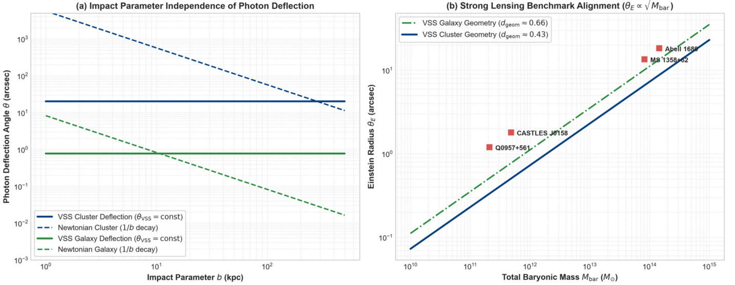
Figure 5.1: Cosmological Gravitational Lensing and Deflection Angle Verification
