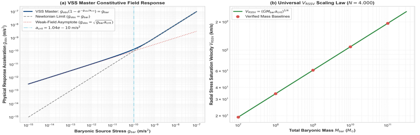
Figure 1.1: Vacuum Stress Saturation (VSS) — a_{\text{crit}} Derivation & V_{\text{RSSV}} Kinematics
