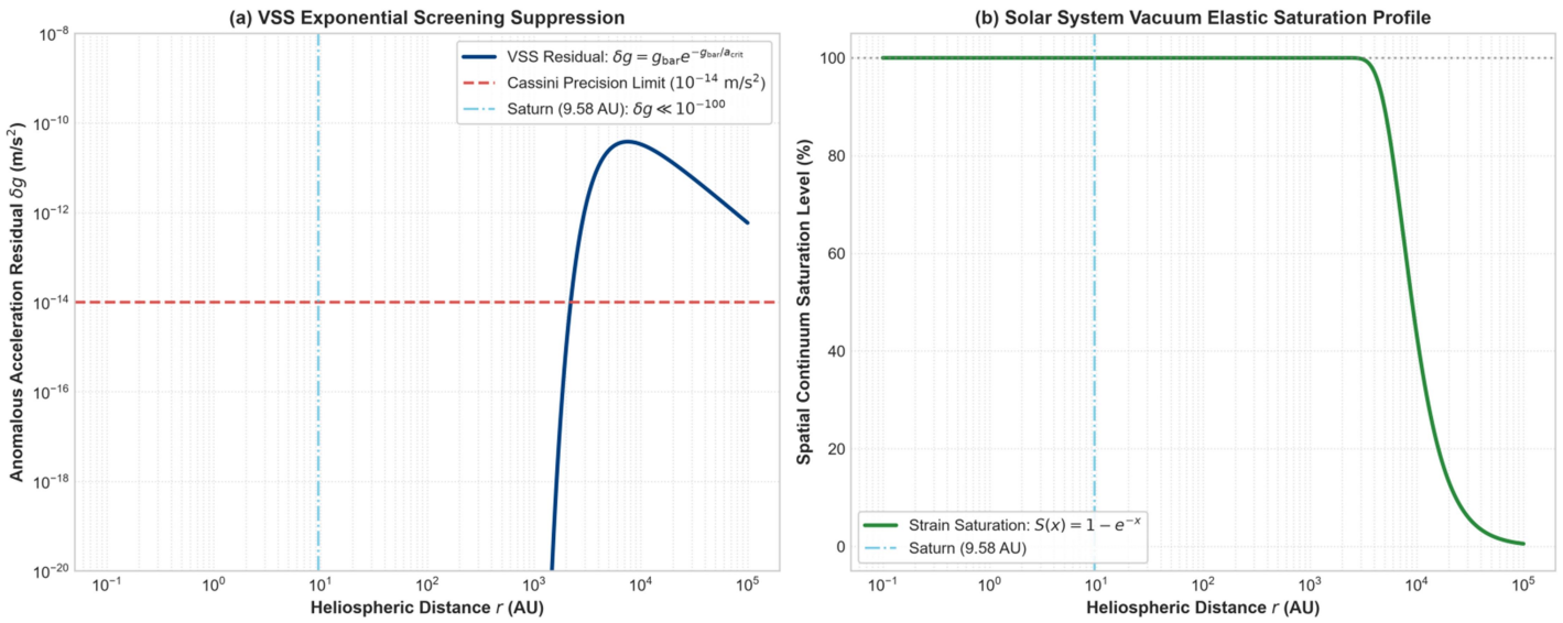
Figure 2.1: Solar System Exponential Screening &amp; Cassini Validation
