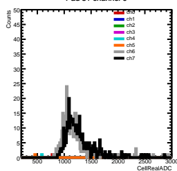
Pad 81 channel 0
