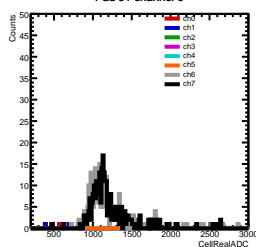
Pad 91 channel 0
