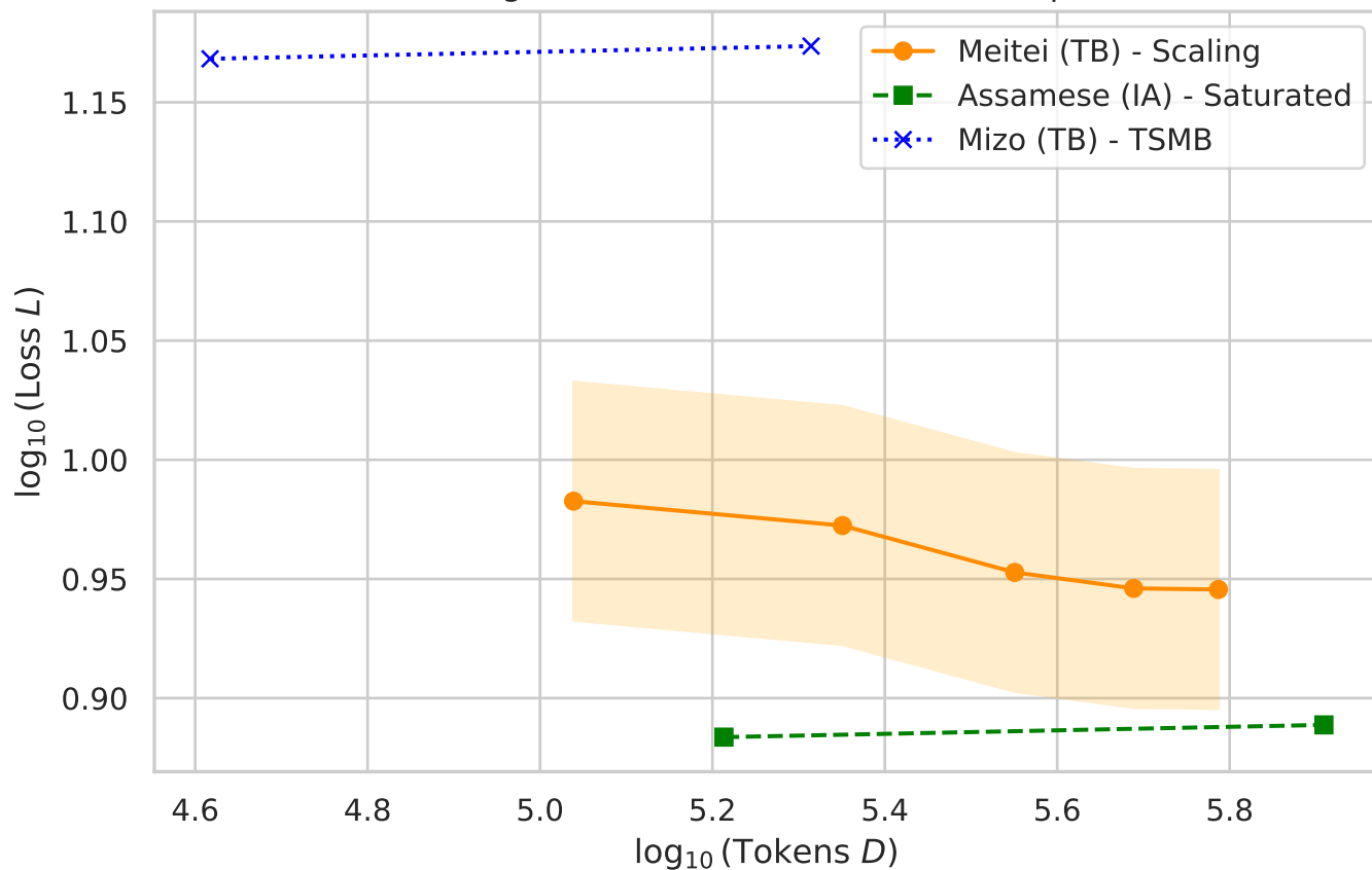
Scaling Law Frontier with 95% Bootstrap CIs
