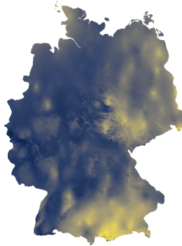
Precip. Seasonality
