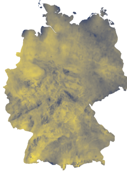
Precip. Seasonality
