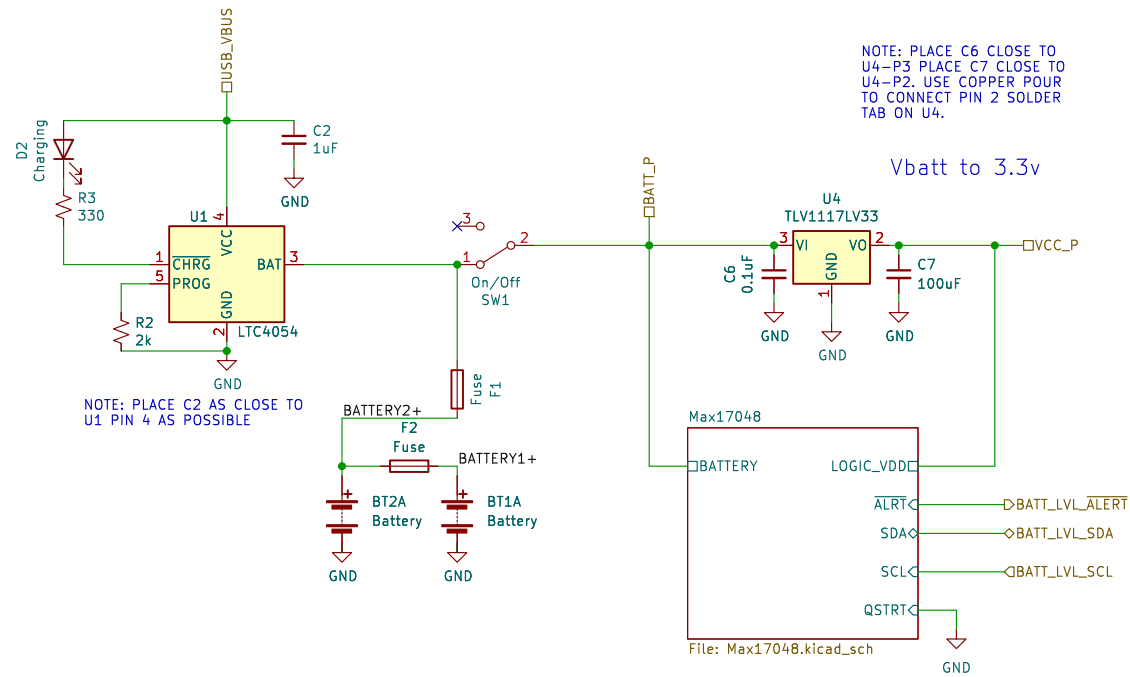
Power and Charge Curcuit
