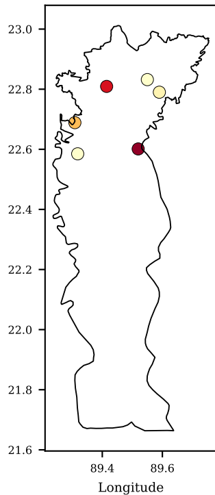
Random Forest
