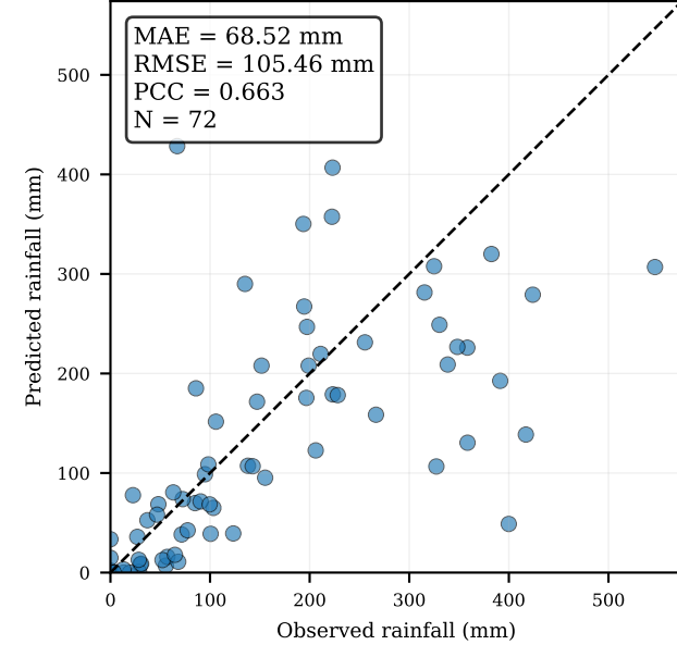
LightGBM
