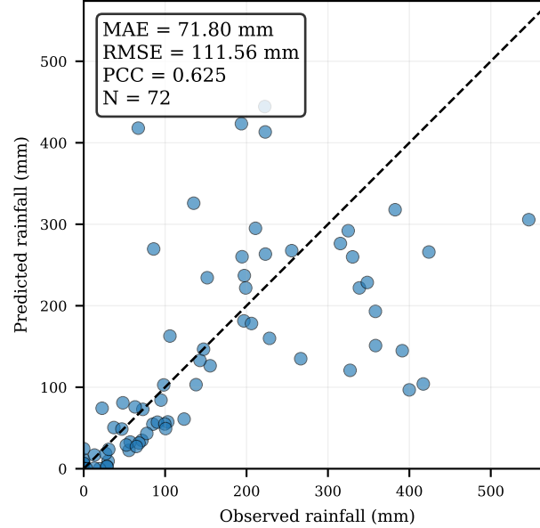
XGBoost
