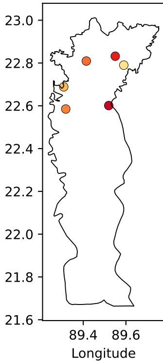
XGBoost
