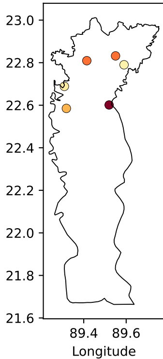
Random Forest
