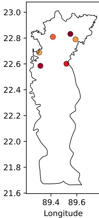
LightGBM
