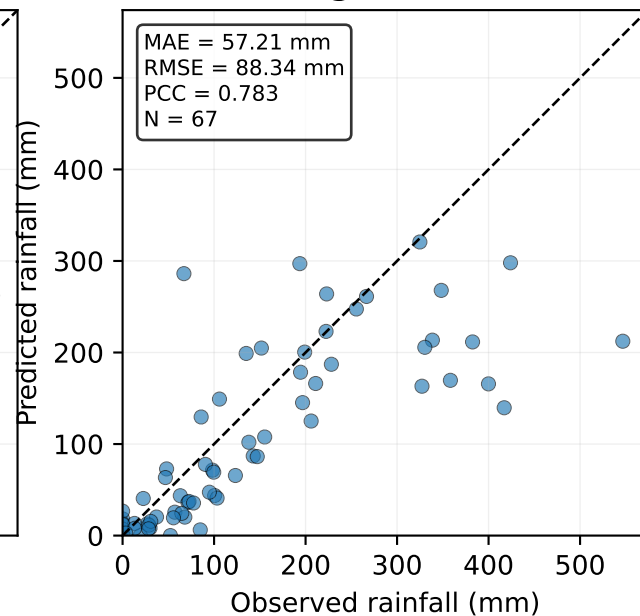
LightGBM
