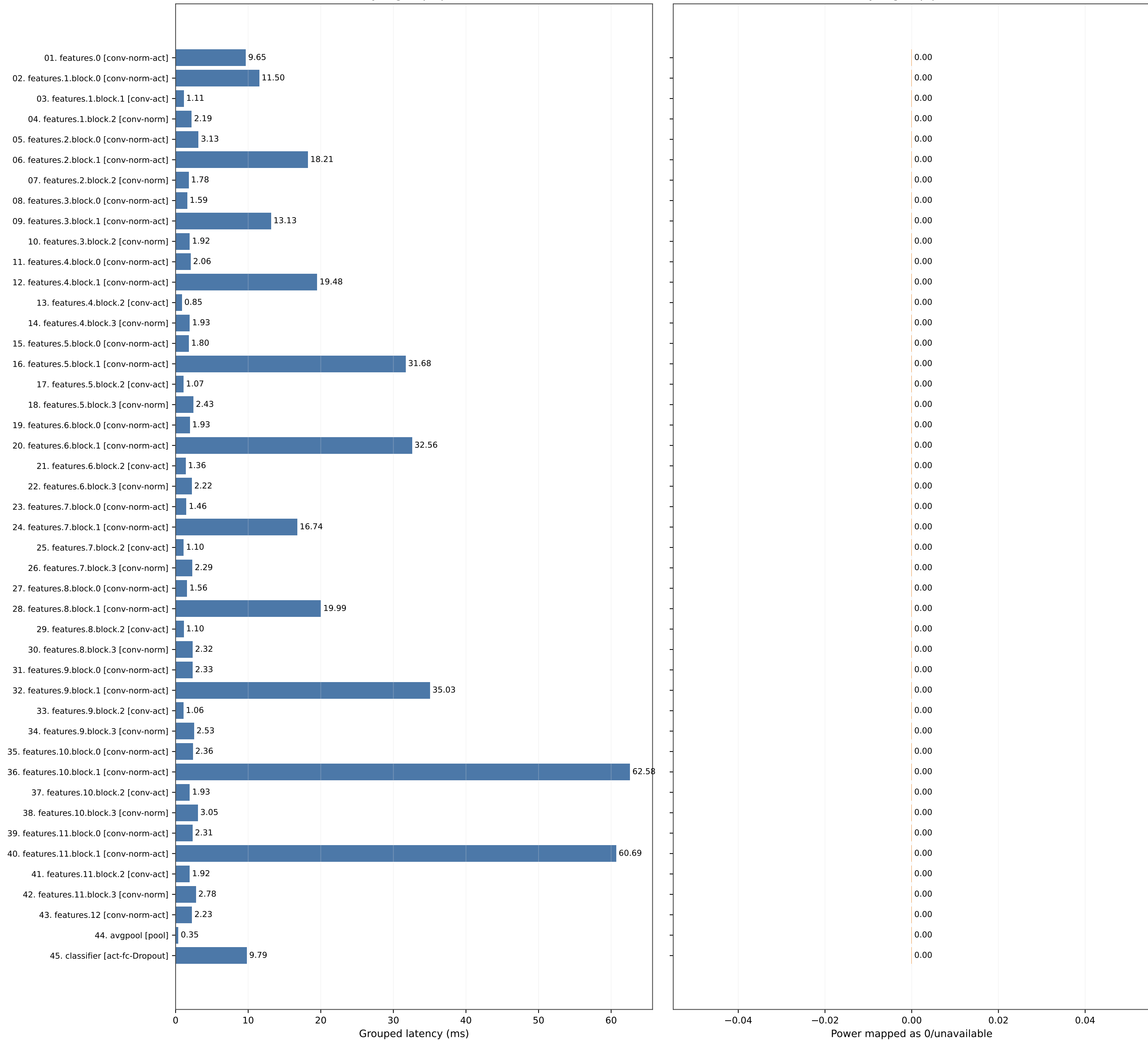
Layer group speed
