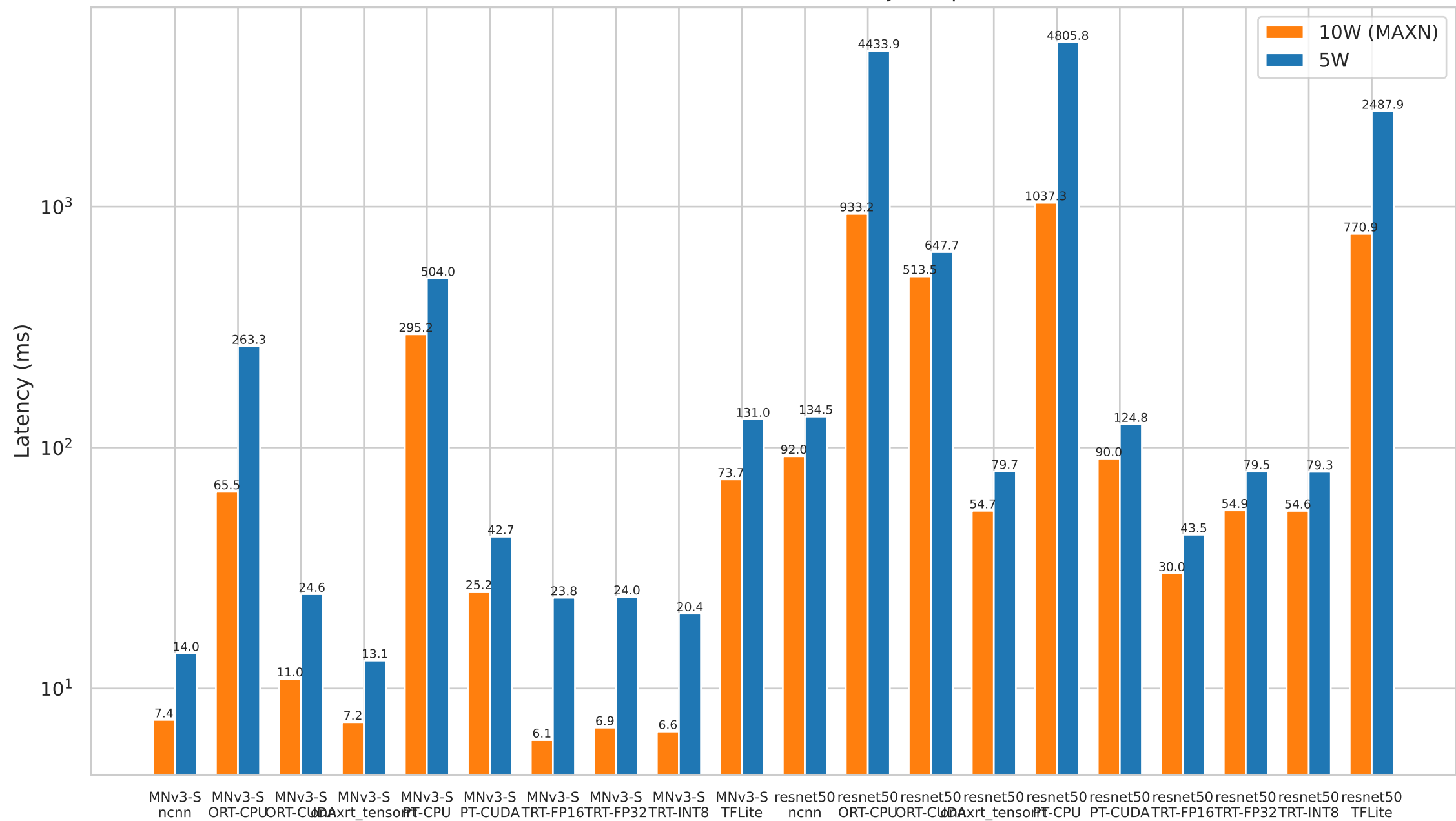
5W vs 10W Mode: Inference Latency Comparison
