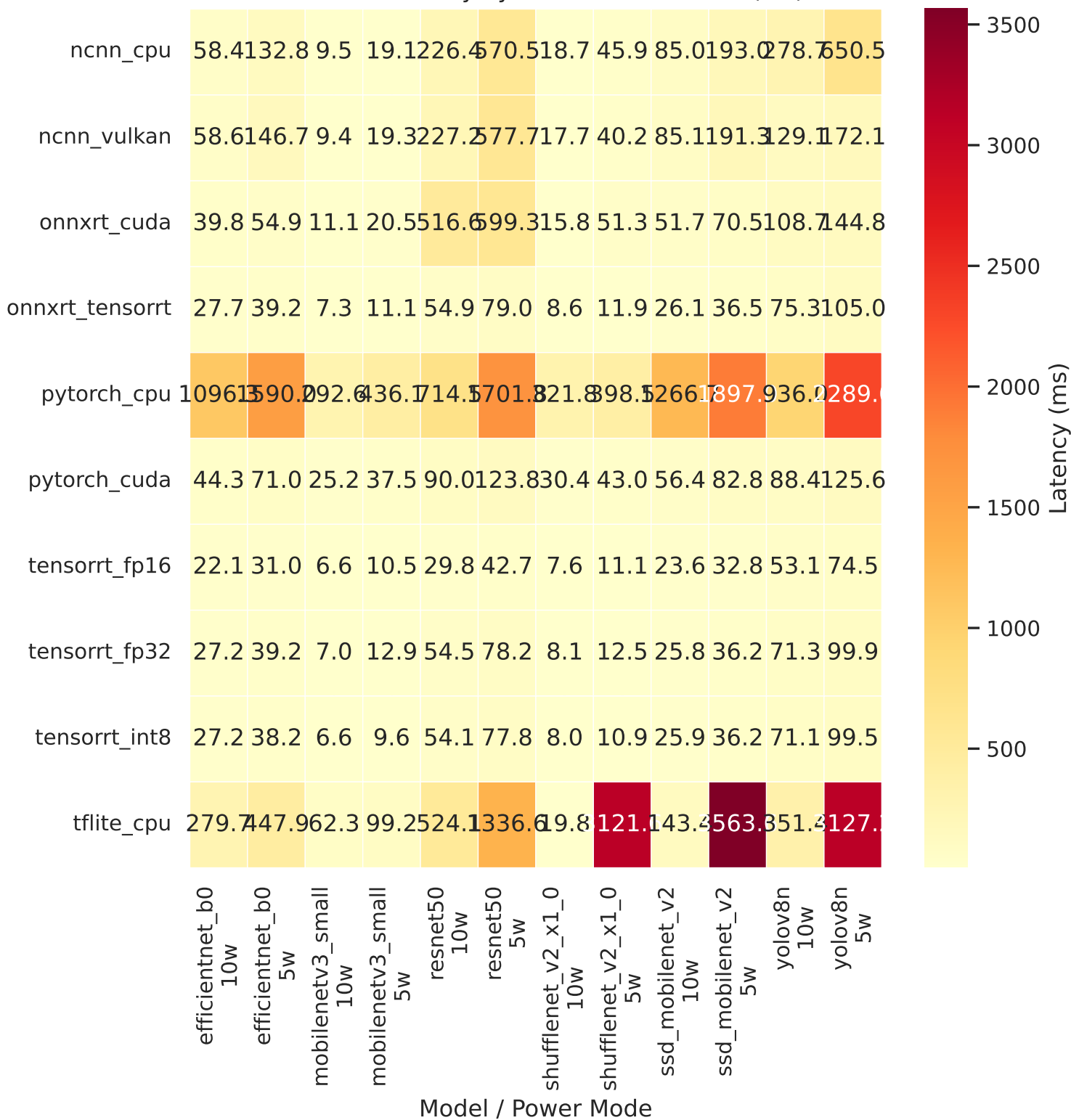
Inference Latency by Runtime and Model (ms)
