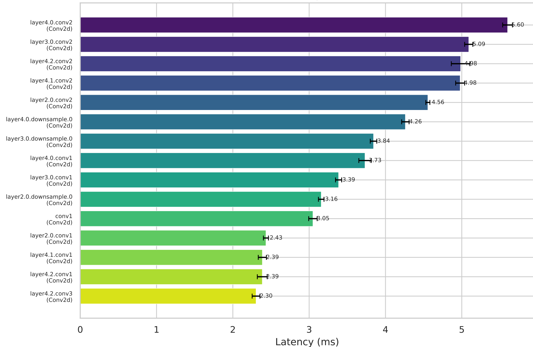
Top-15 Slowest Layers: resnet50
